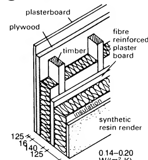
⑨ Timber panel construction 0.14-0.20 W/(m 2 ·K)
